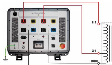
Connecting TWR-B to a single-phase autotransformer
