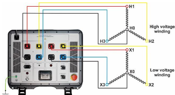
Connecting TWR-B to a three-phase transformer
