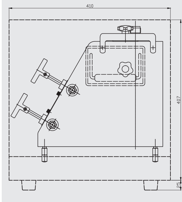
Side view (with case dimension)
