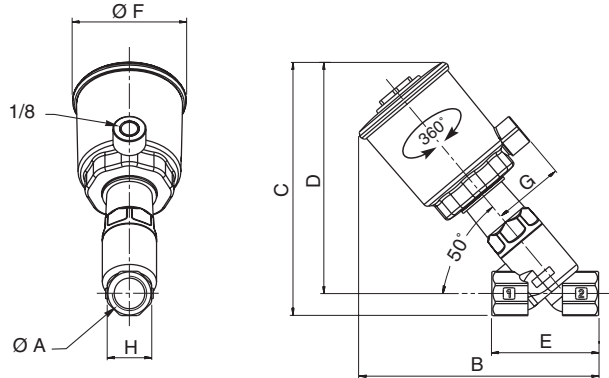
TYPE 01-02 32 and 50 mm operators Fluid entry: under the disc at 2 above the disc at 1
