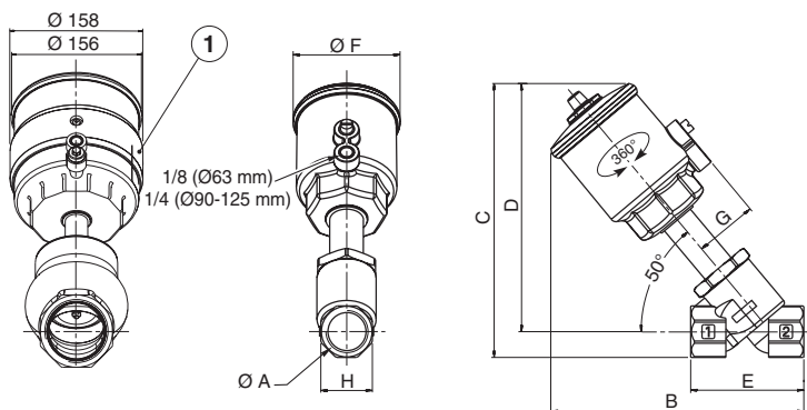
TYPE 03-04-05 63, 90 and 125 mm operators Fluid entry: under the disc at 2 above the disc at 1
