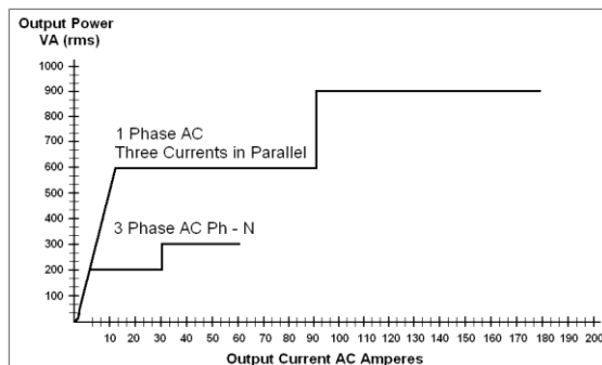
Figure 2 Current Output Power Curve
