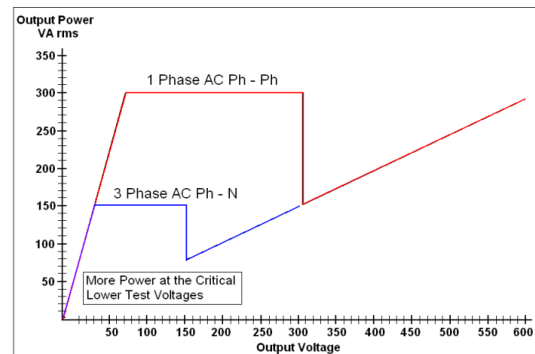
Figure 3 Voltage Output Power Curve
