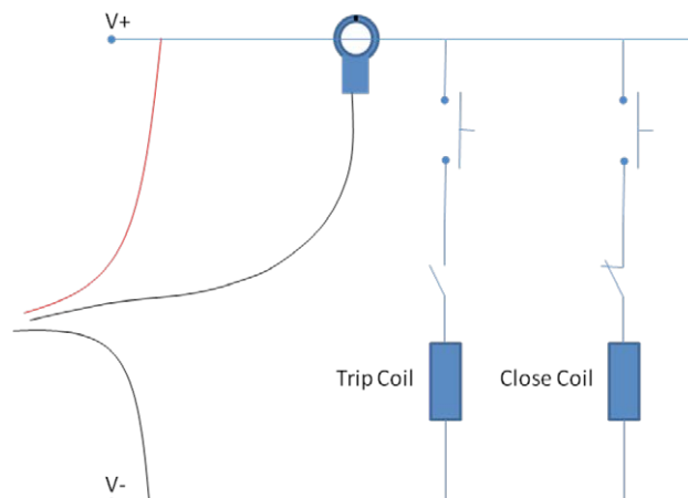
Figure 1 Point for measuring coil current and control voltage
